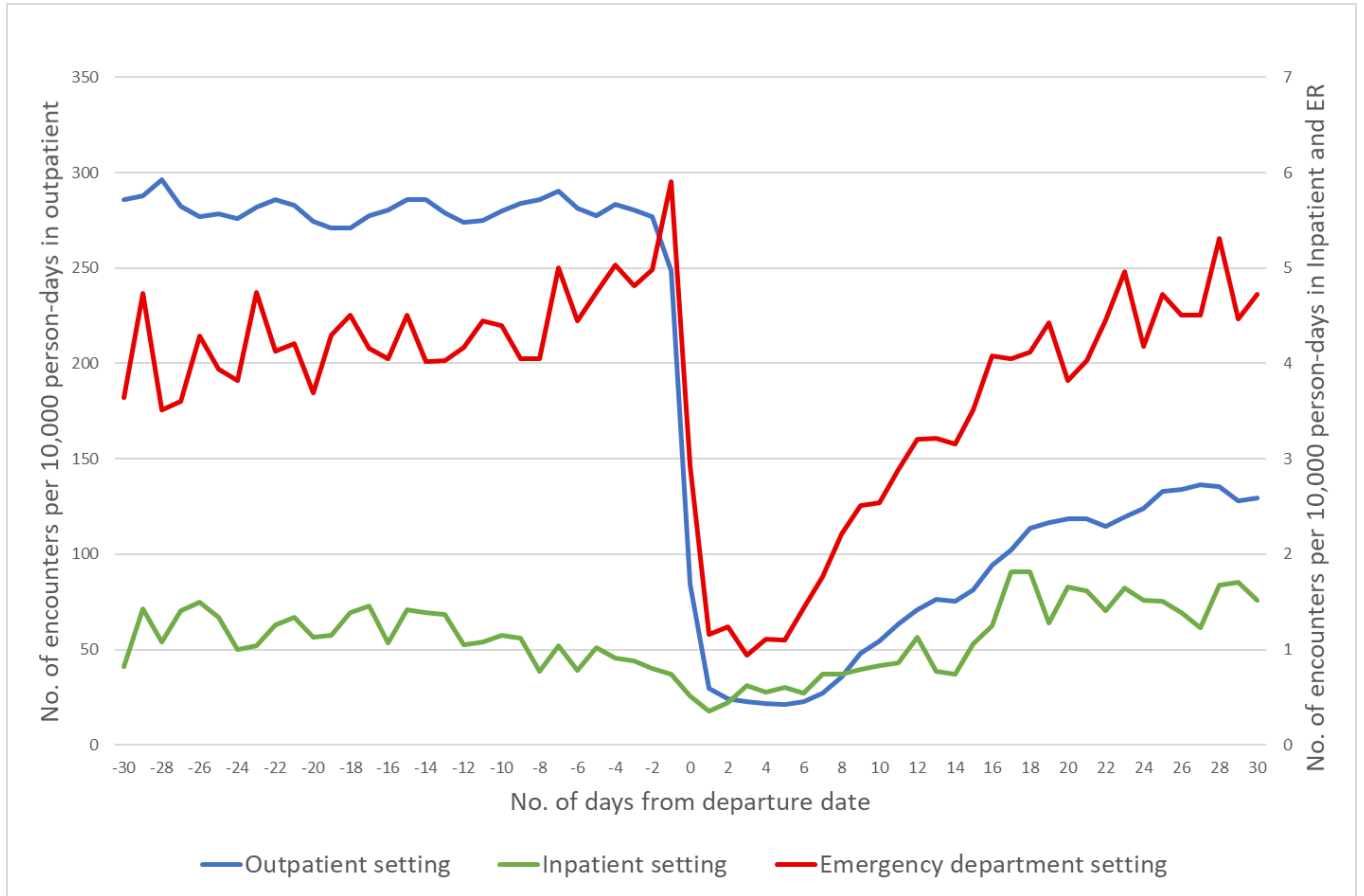
Supplementary Figure 1. Encounter rate before and after travel by care setting
